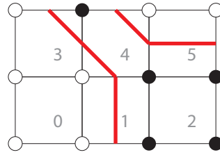
Figure 1. Mesh for contour algorithm examples
